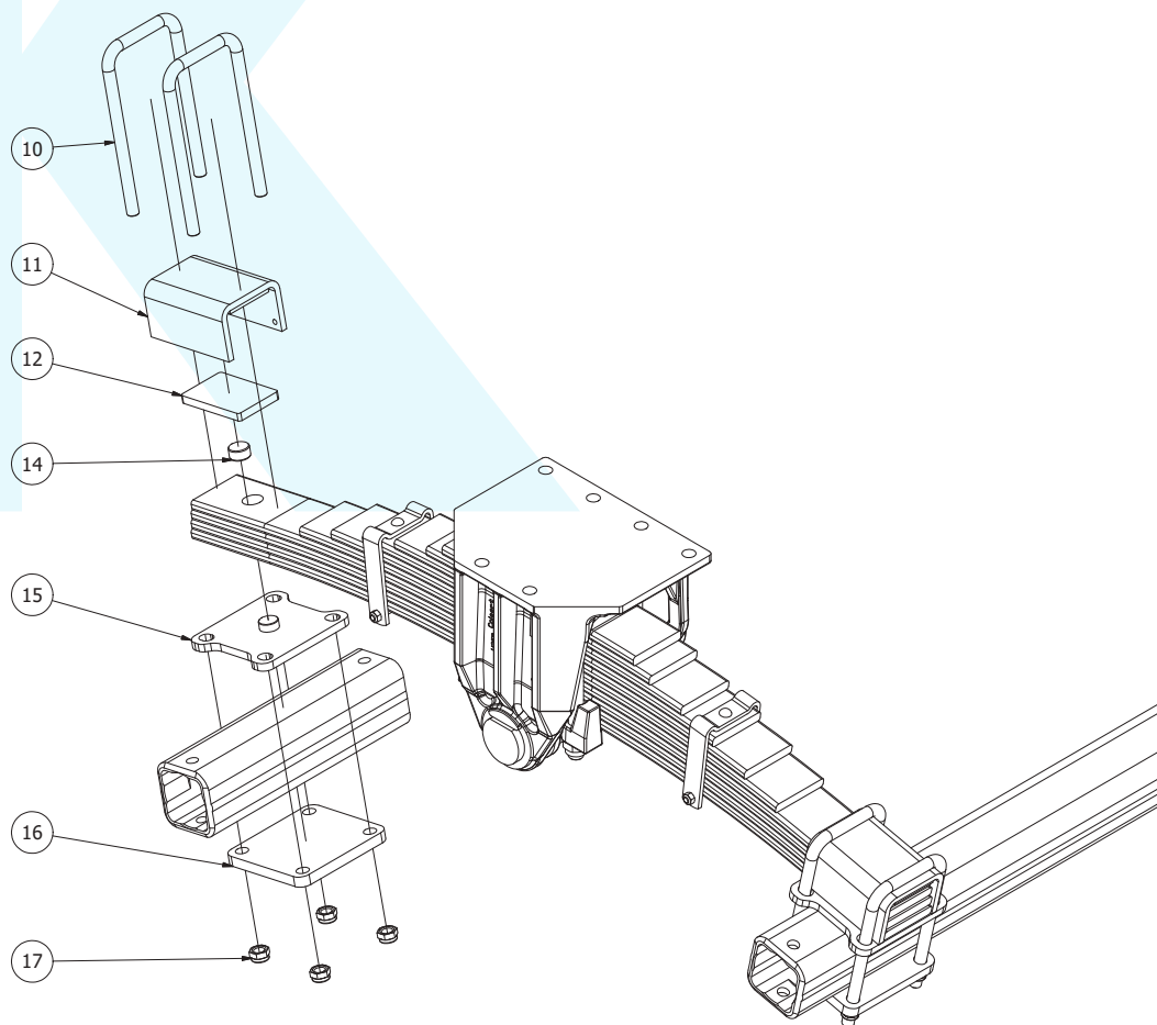
Bridage / Clamping type P
