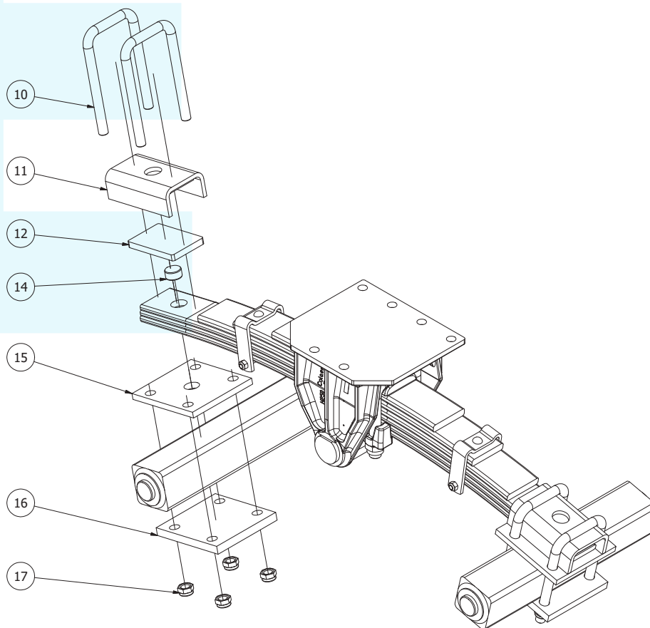
Bridge / Clamping type P
