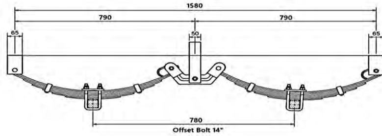
Tandem Spring Set
