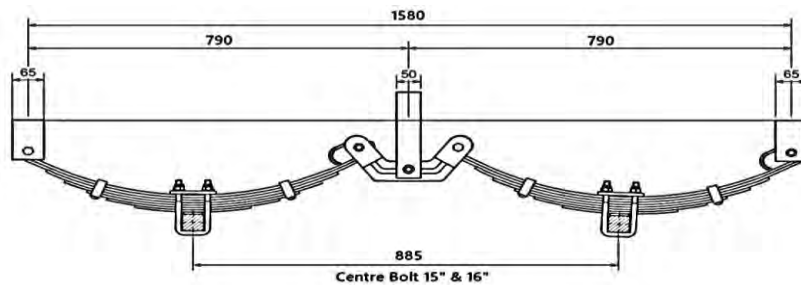
Tandem Spring Set
