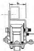
Tandem Suspension Set (Pair)
