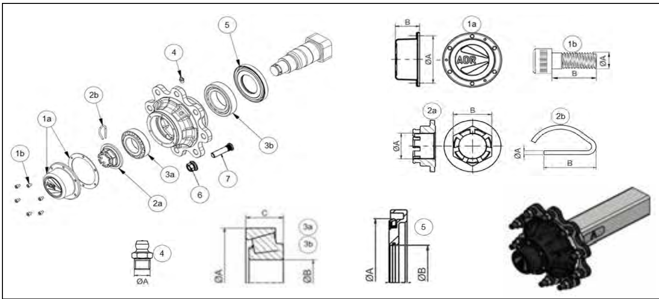
100mm Square 10/335 (ADR Part. 1100)
