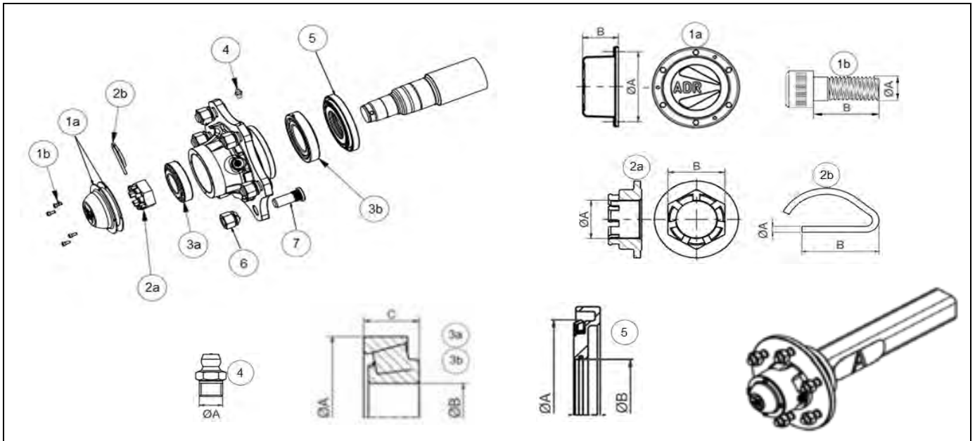
50mm Square 5/140 (ADR Part. 1500)
