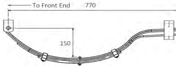
Single Spring Set (Pair)
