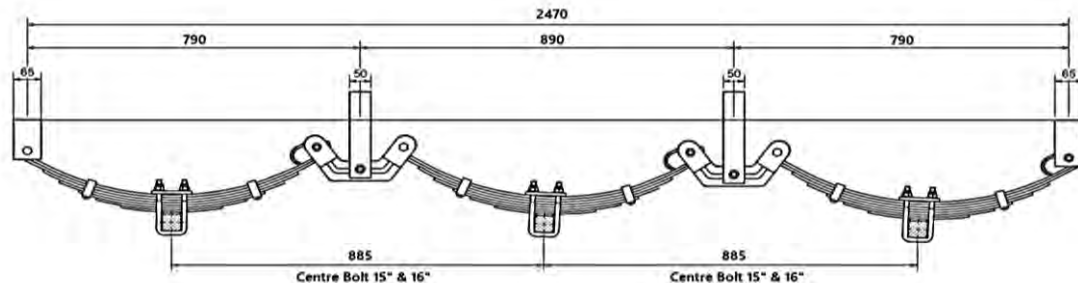
Triple Spring Set
