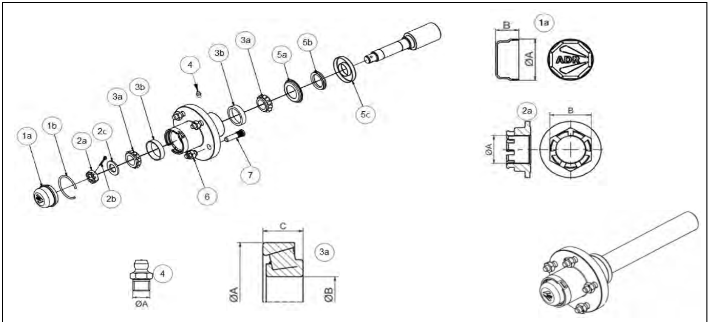
39mm Round 5/107.95 HT (ADR Part. 1416)
